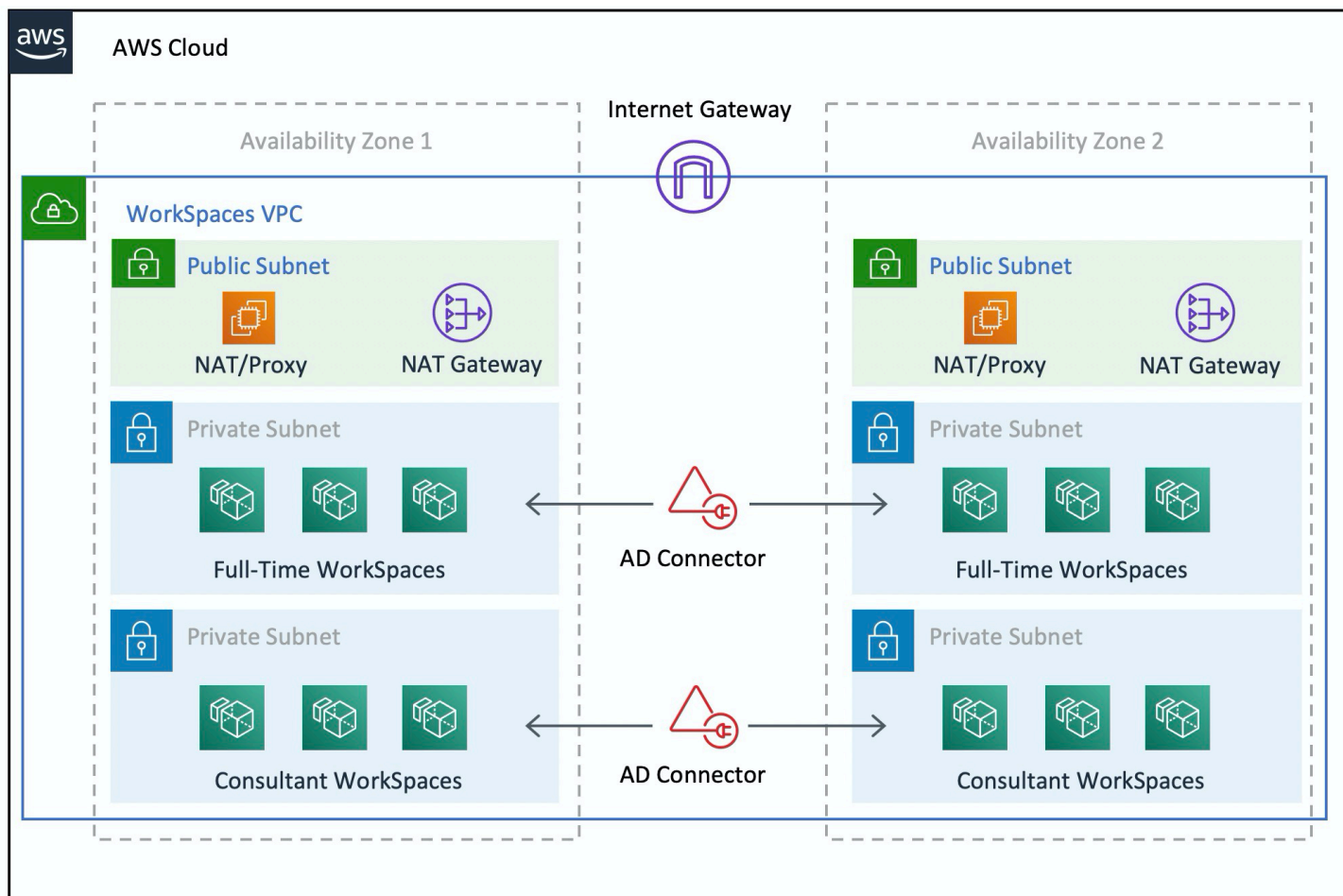
Abbildung 3: High-Level-VPC-Design
